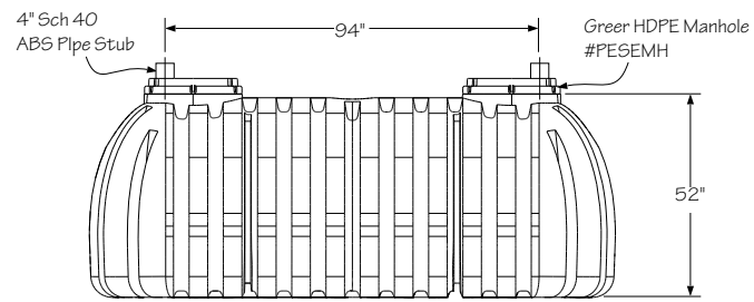
Interior Plumbing - 1250 Gallon Low Profile, 4' Max Burial, Polyethylene Septic Tank
